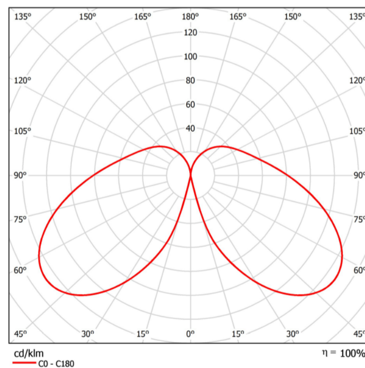
Distribution curve KARIN 900 LED
